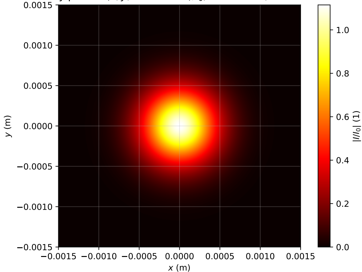
Intensity profile I(x, y, z = 0.398m)/I_0 , P_{in}=1.0P_{cr} , artificial time
